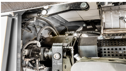
The VarioDirect drive allows the shaft to increase torque, reverse and start under load.
