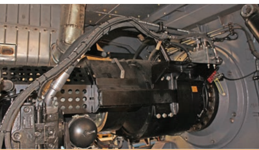
The shaft is directly driven by the engine for maximum torque, power and efficiency.
